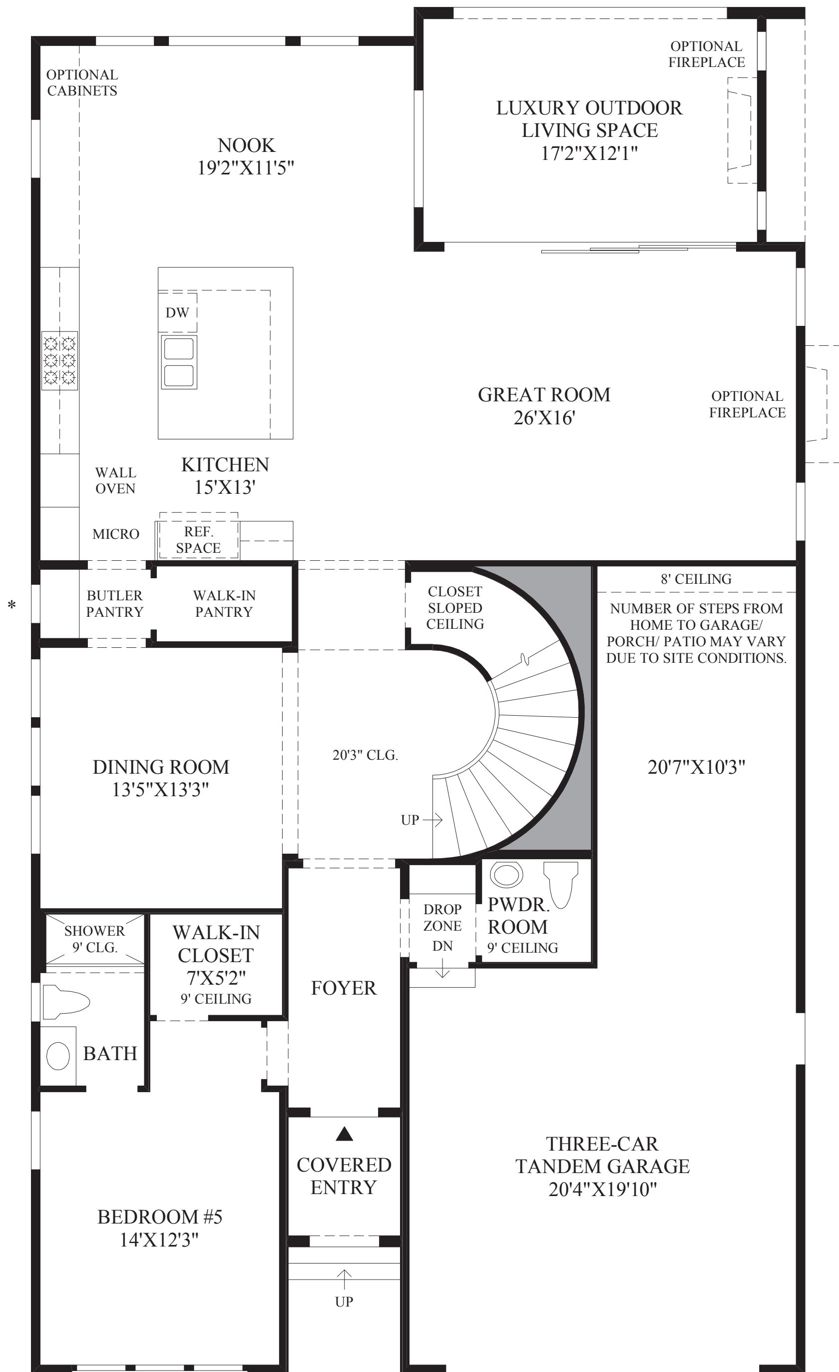
First Floor TUSCAN EXTERIOR DESIGN SHOWN
